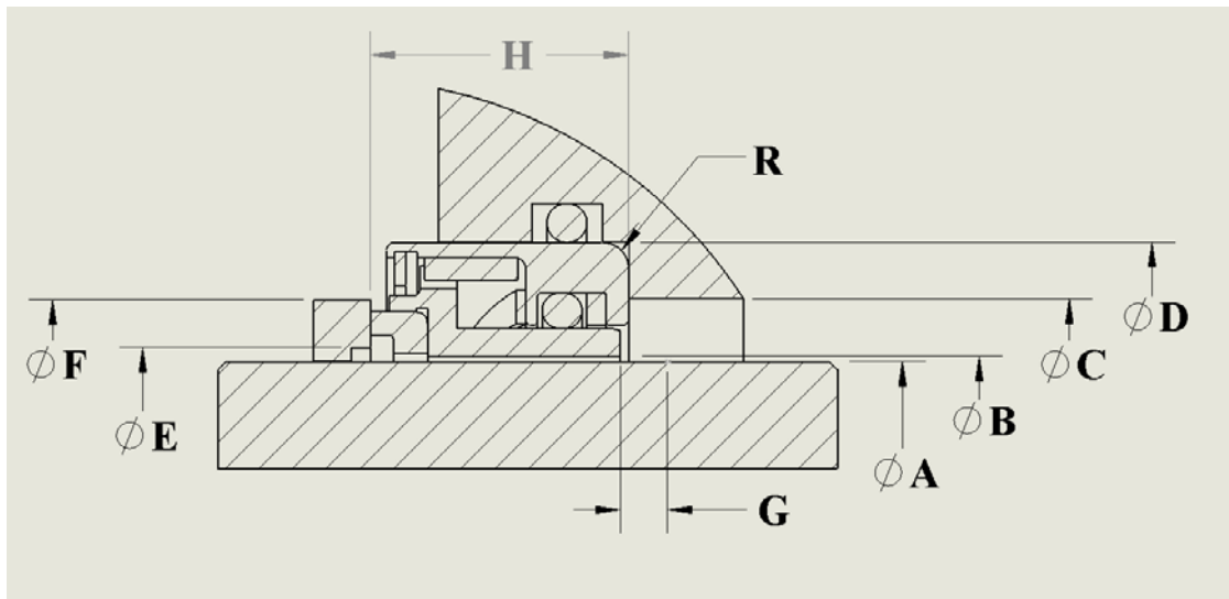
Type 14 Seal Design
