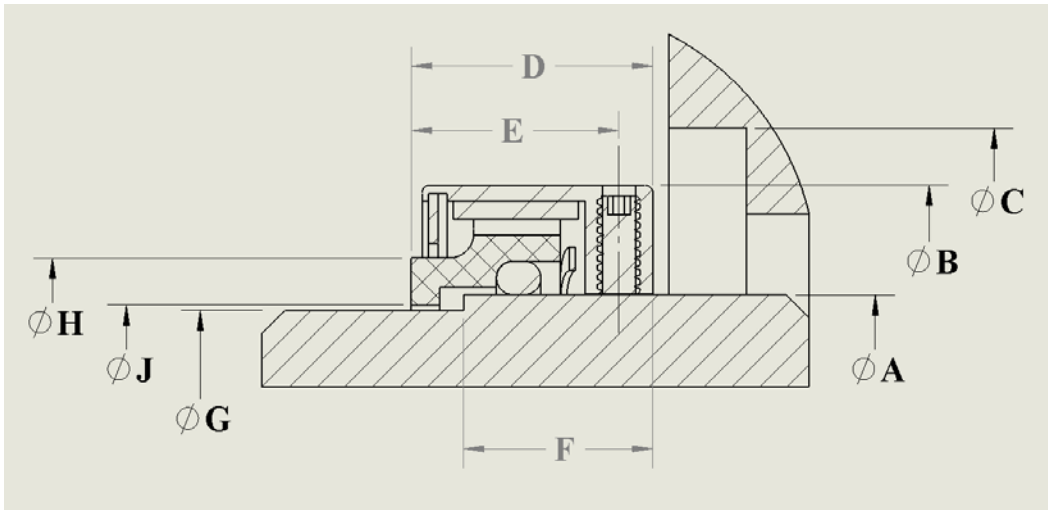
Type 30B Seal Design
