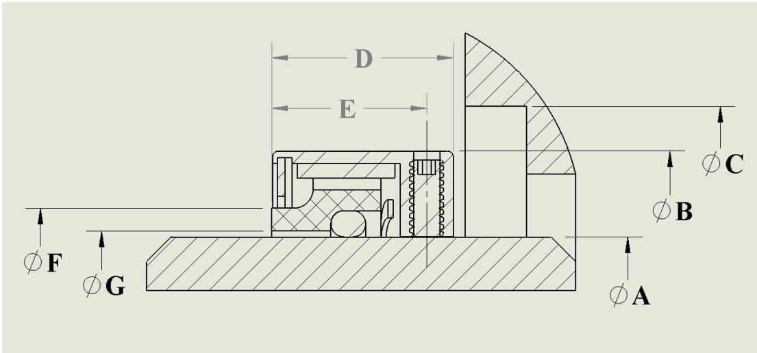
Type 30 Seal Design
