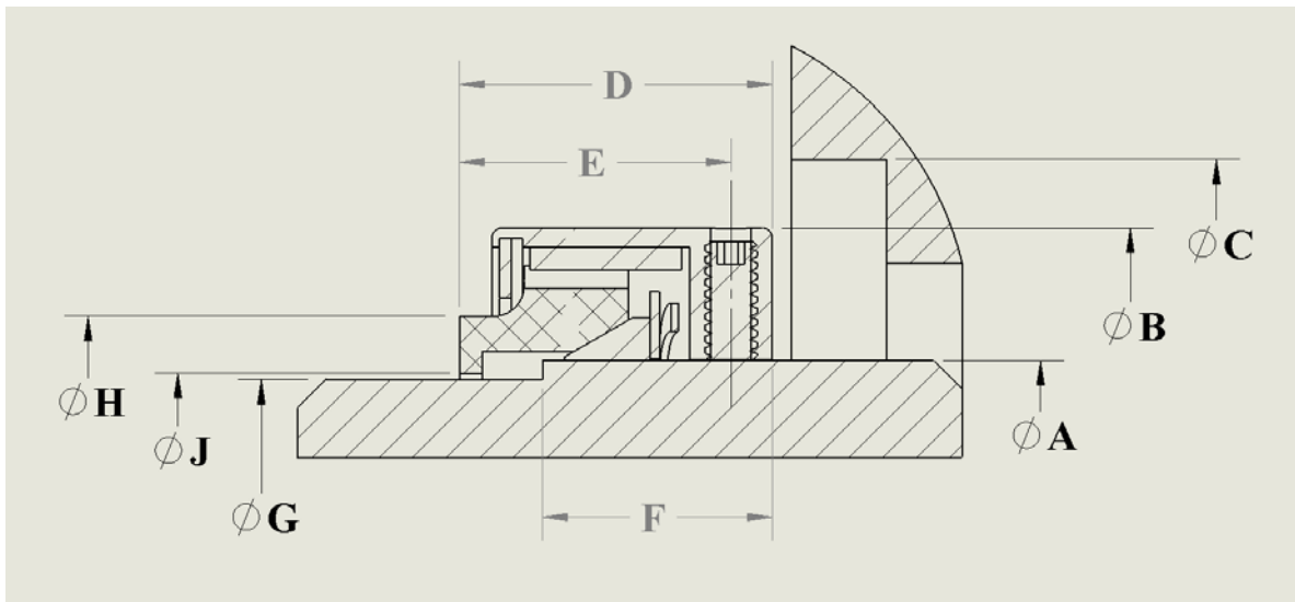
Type 39B Seal Design
